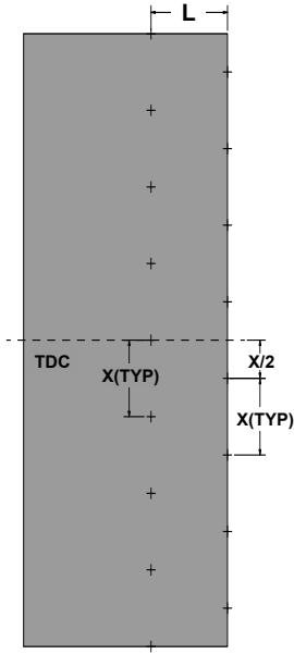
FIGURE 4-1 PIPE OD UNROLLED FOR VISUAL
