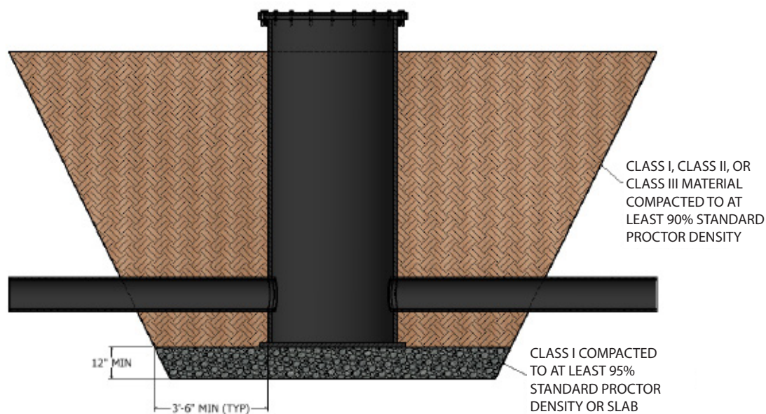
Figure 5-2: Typical Installation Recommendations
