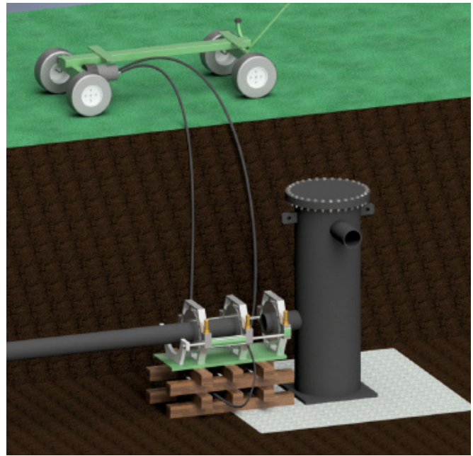
Figure 5-1: In-Ditch Fusion Setup
